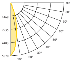
Candle Power Distribution Curve
